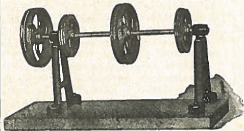
Transmission 4 poulies.
